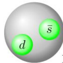
Pion chargé \pi^+
