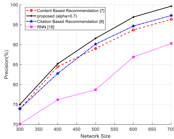
Fig. 9. The precision criterion for different dimensions of the citation network.
